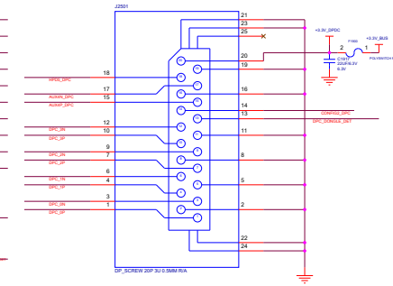
Anney: Change to SMT POOL SYMBOL
